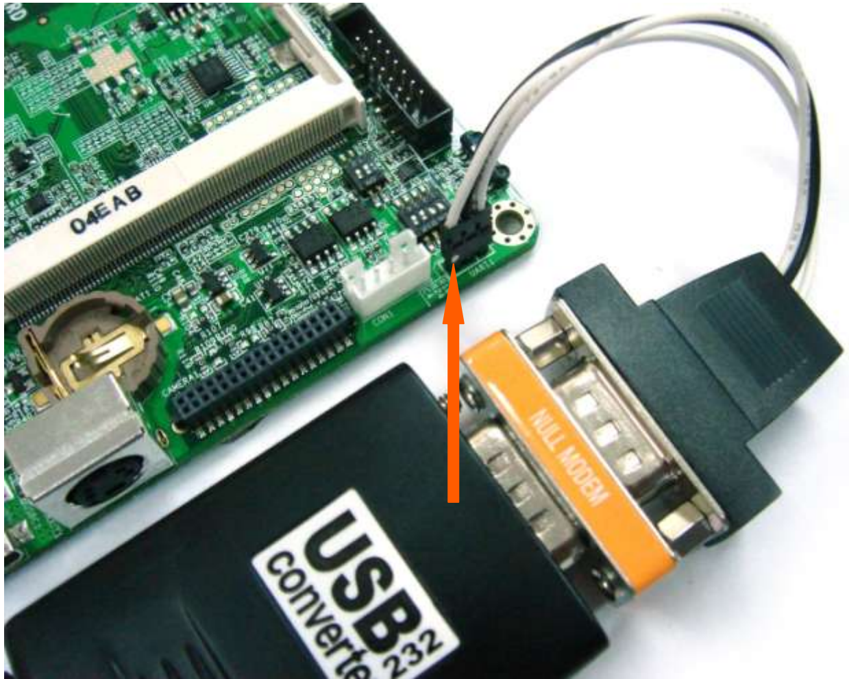
Figure 37: The cable (RS-232 to USB) with null-modem-block connected to the UART1 (5) connector (see orange arrow for position of the white dot (note: turned 180 degrees))
