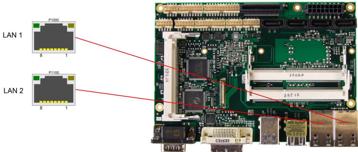
Pinout LAN 10/100/1000:
