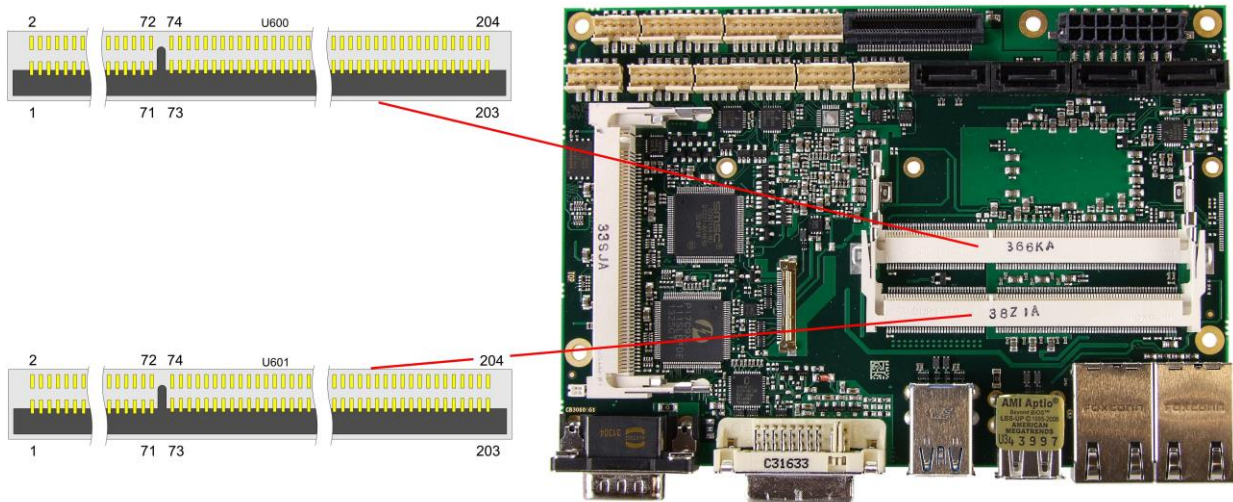
Pinout SO-DIMM204:
