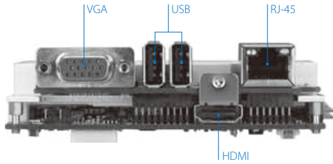
I/O of EPIA-P720 Board with P720-A
