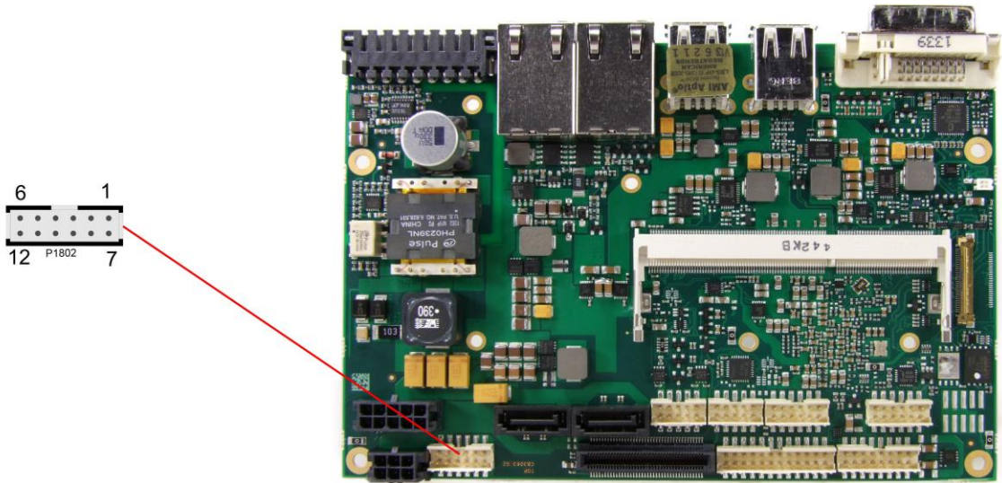
Pinout Molex connector 2x6:
