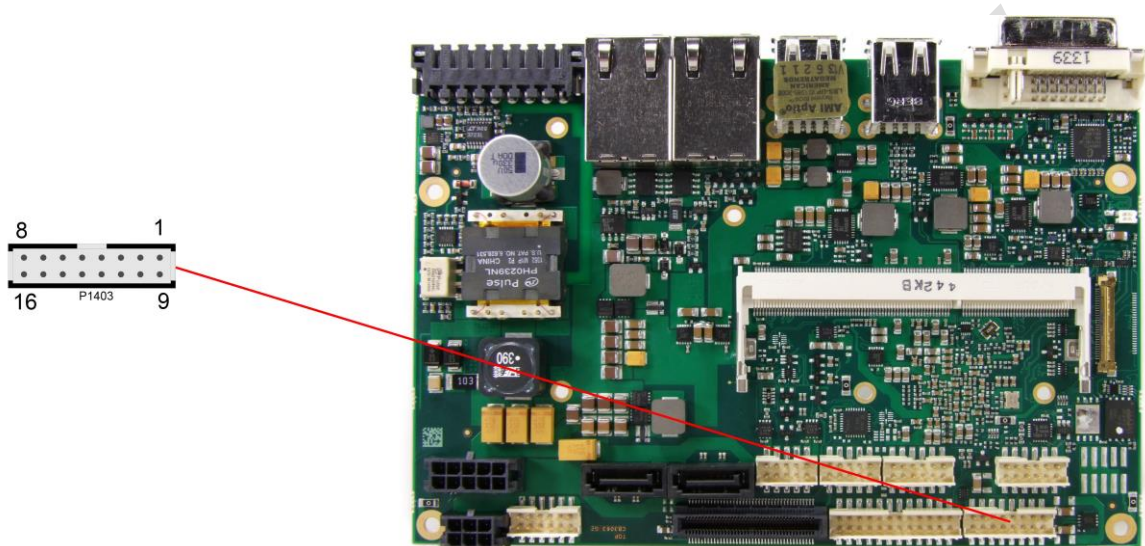
Pinout USB
