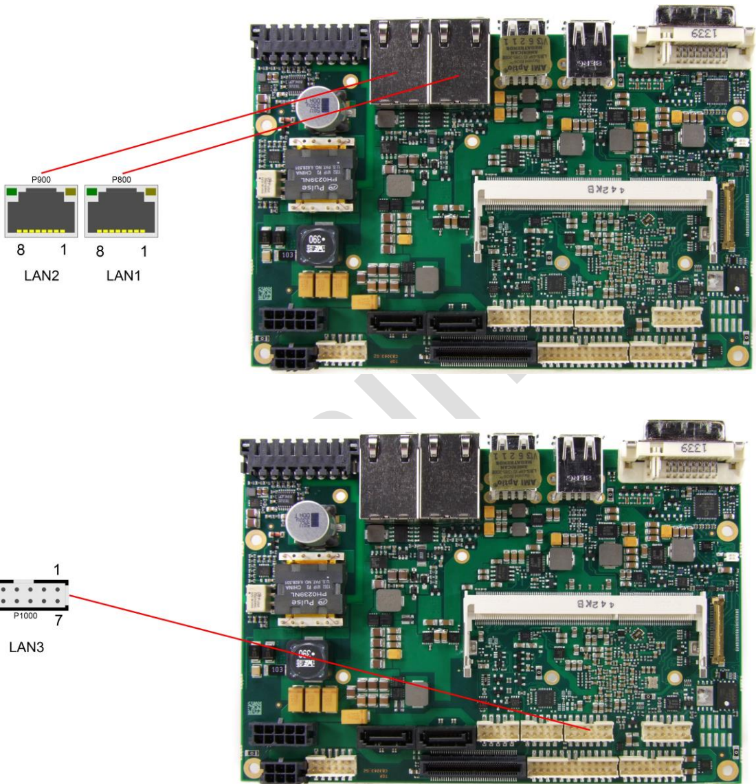
Pinout LAN 10/100/1000:
